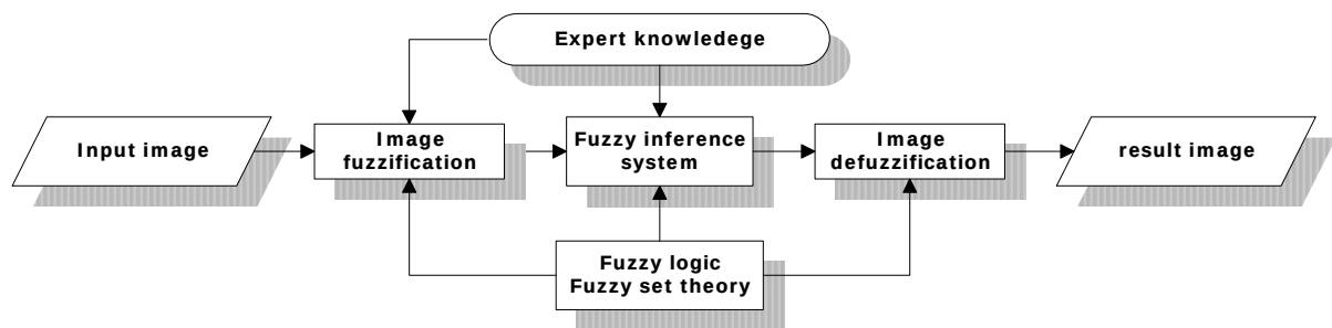
Fig. 2 The general structure of fuzzy image processing
